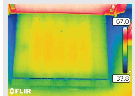
BEFORE: Hot or cold air can easily transfer through perimeter gaps.
